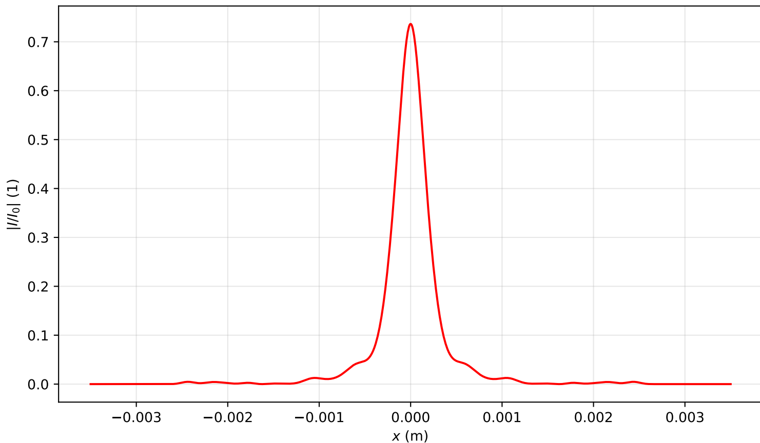
Intensity profile I(x, y = 0, z = 2.866)/I_0 , P_{in}=4.0P_{cr} , artificial time
